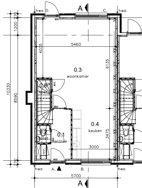
Begane grond (0.000+)
